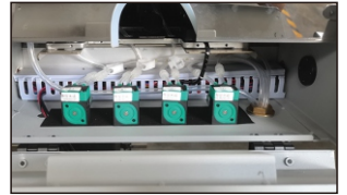
Ink pump
